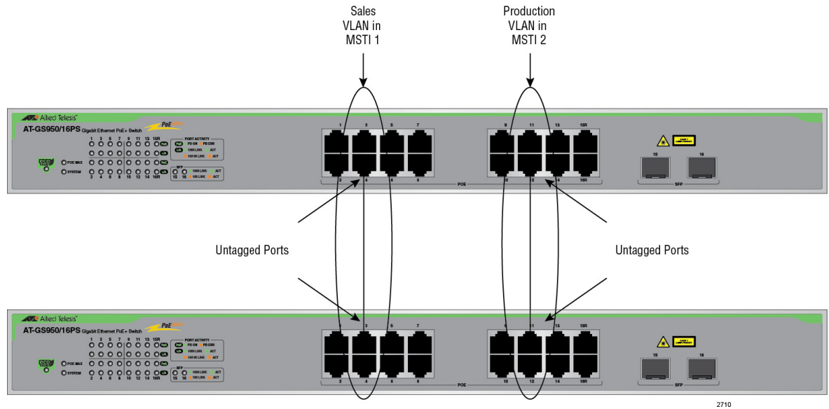
Figure 140. MSTP Example of Two Spanning Tree Instances
